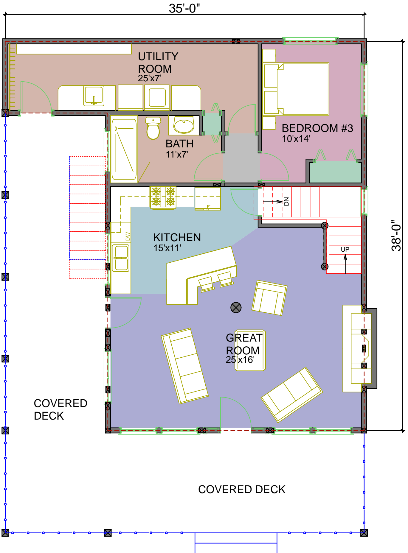
FIRST FLOOR PLAN AREA: 1056 SQ. FT.
