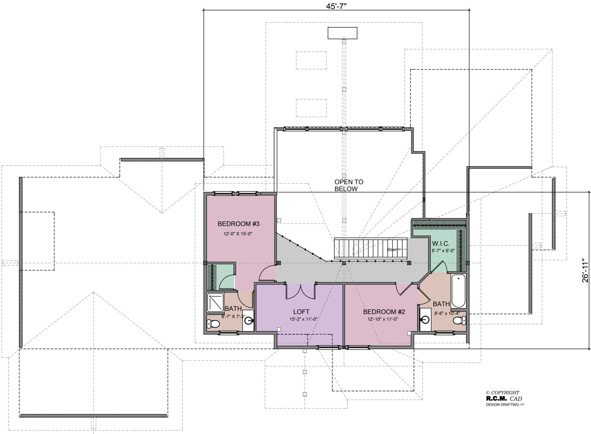
SECOND FLOOR AREA: 804 SQ. FT.
