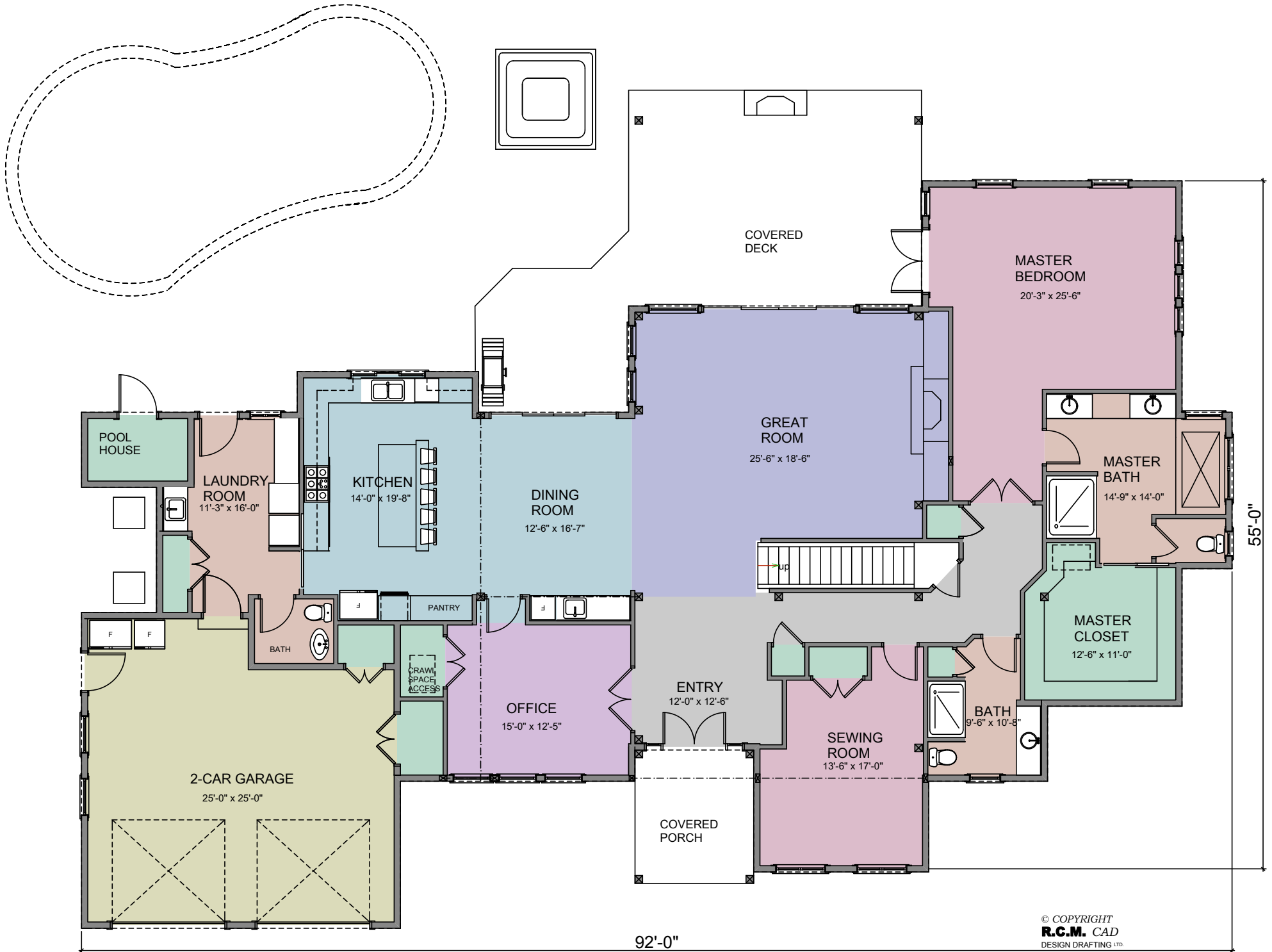
FIRST FLOOR PLAN AREA: 2941 SQ.FT.
