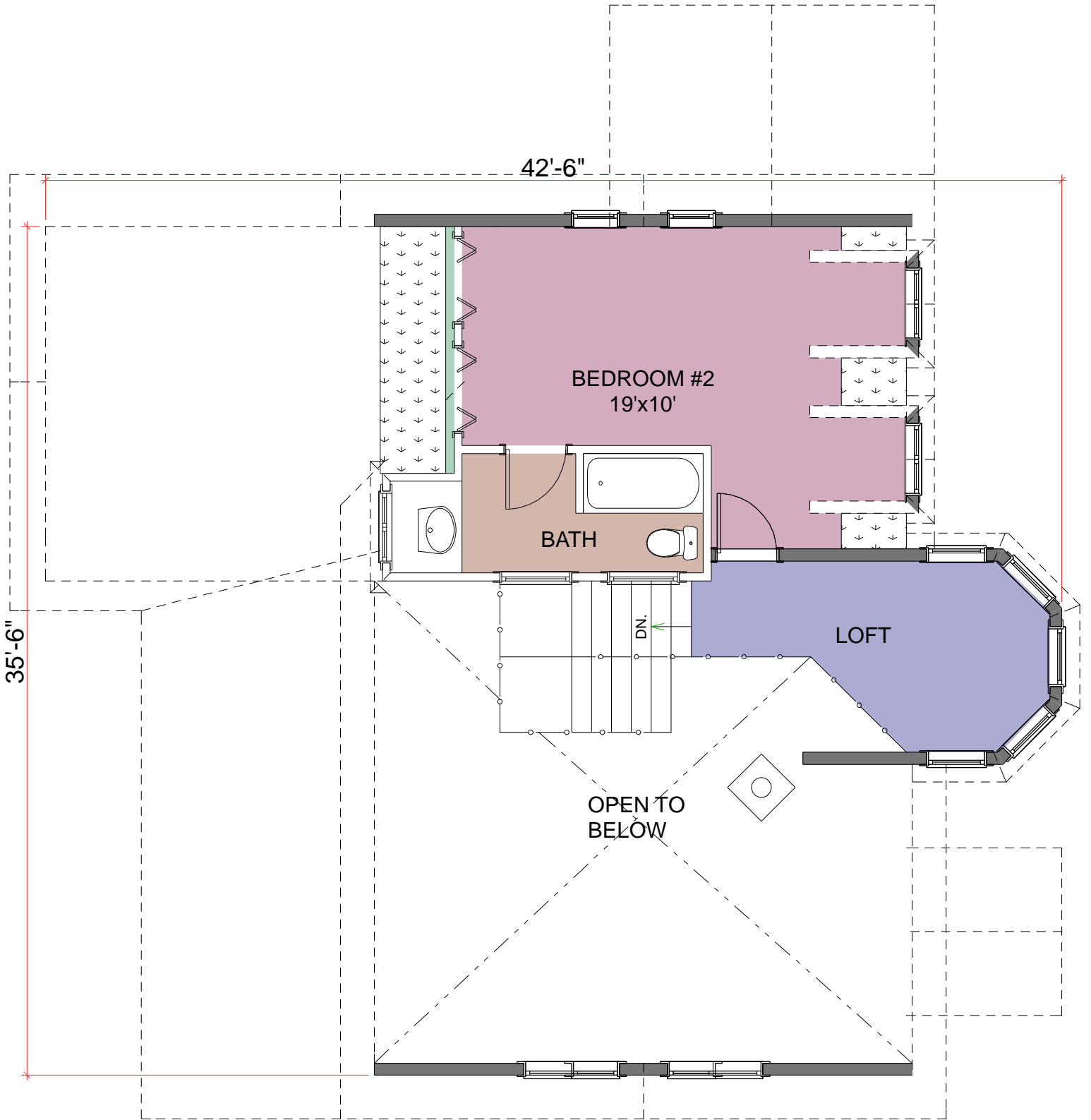
SECOND FLOOR PLAN AREA: 387 SQ. FT.
