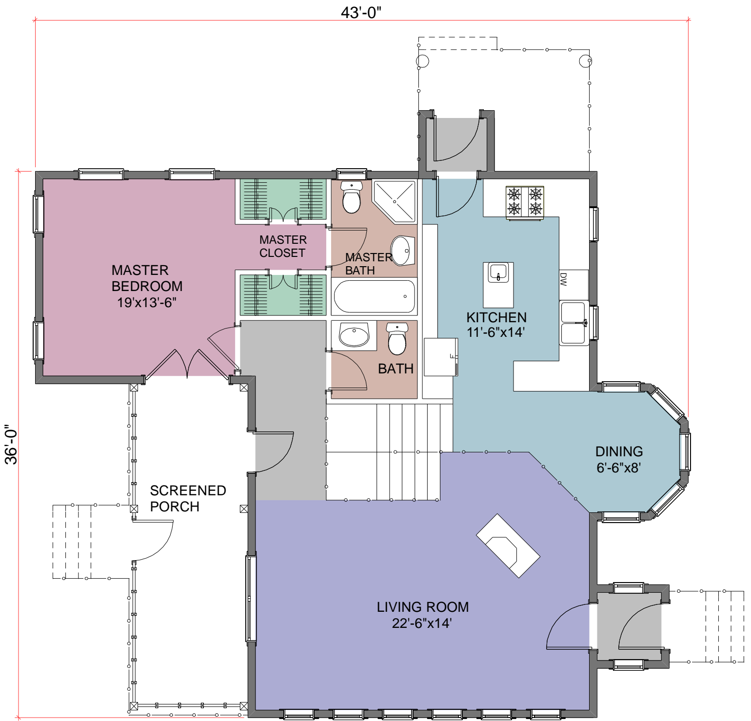
FIRST FLOOR PLAN AREA: 1016 SQ. FT.
