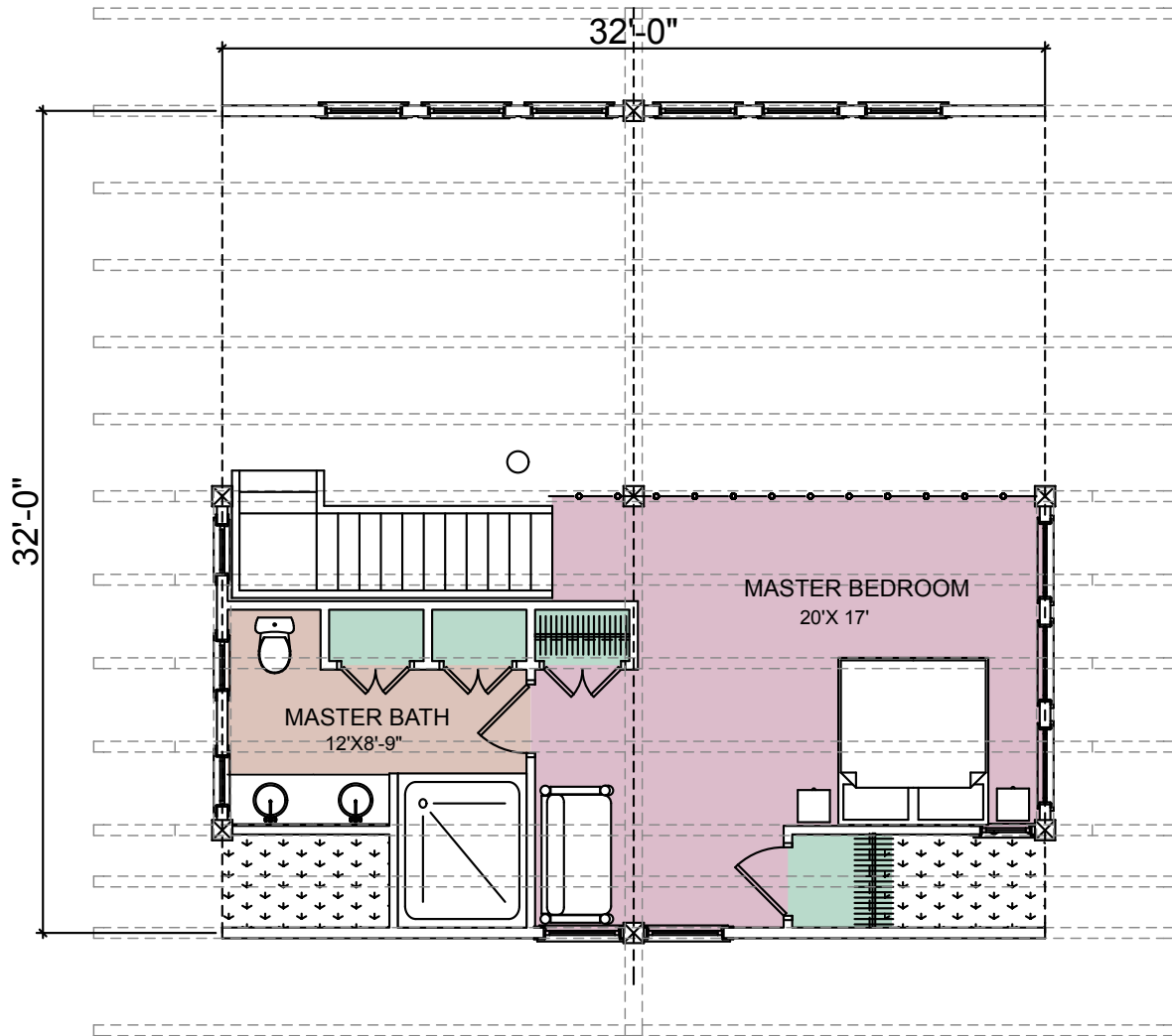
SECOND FLOOR PLAN AREA: 500 SQ. FT.
