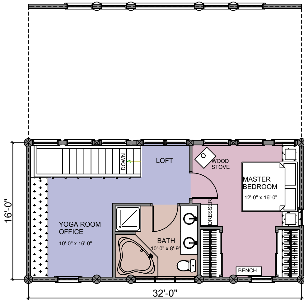
SECOND FLOOR PLAN AREA: 405 SQ. FT.
