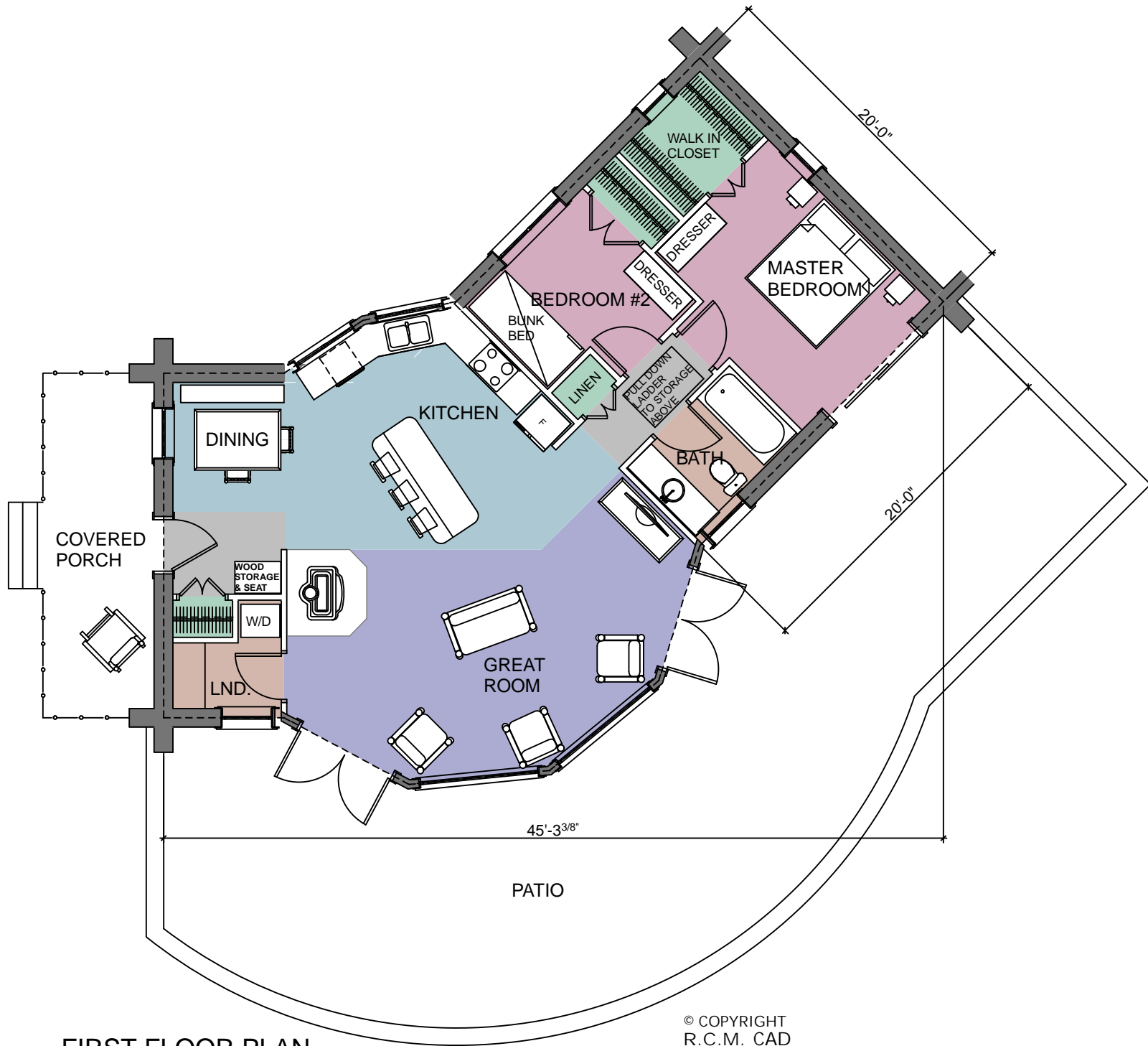
FIRST FLOOR PLAN AREA: 1040 SQ.FT.
