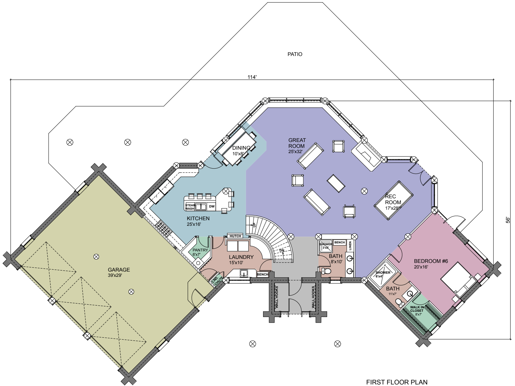
FIRST FLOOR PLAN AREA: 2637 SQ.FT.
