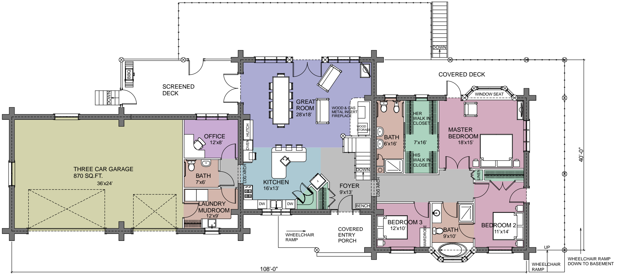
FIRST FLOOR PLAN AREA: 2260 SQ.FT.
