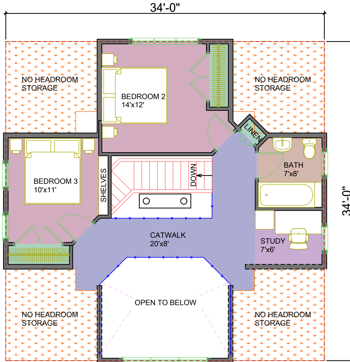
SECOND FLOOR PLAN AREA: 587 SQ. FT.
